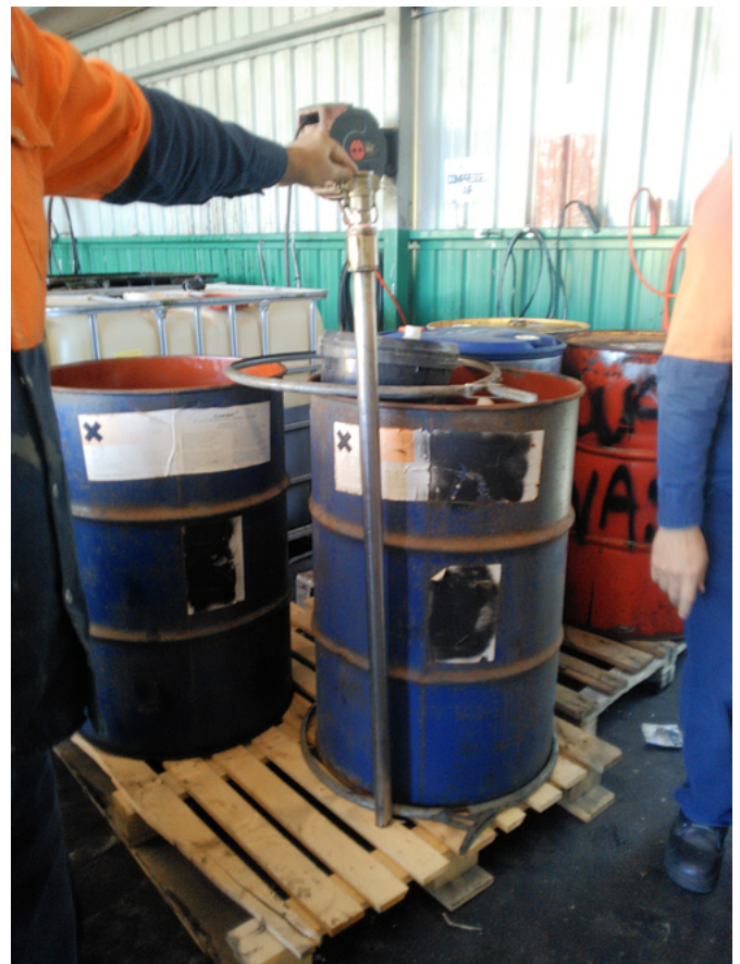
Figure 4 Metal (conductive) pipe for transfer of flammable liquids sufficiently long enough to avoid splashing and generation of static electricity
