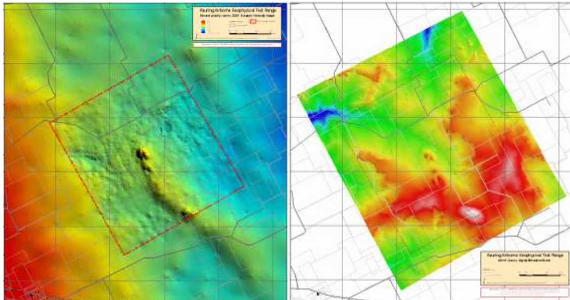
Figure 1: The Kauring Test Range Gravity Bouguer Anomaly image (left) and LiDAR topography (right). In both images, red indicates high values and blue low values. Gravity values range from -210 to -380 gu; elevation from 240 to 360 m.
