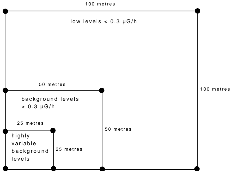
Figure 2.1.: Gamma survey – recommended grid sizes
