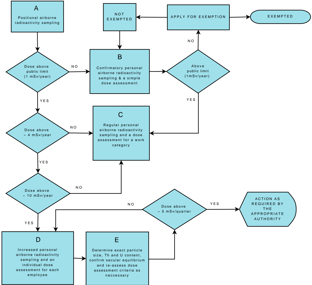
Figure 2.1.: Airborne radioactivity sampling
